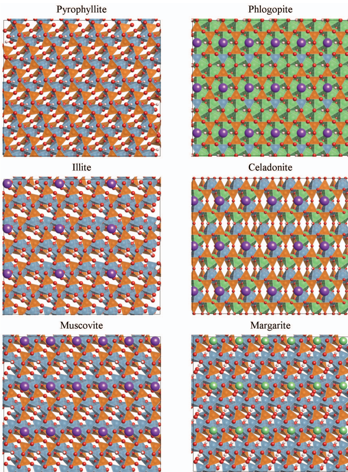
Figure 1. Top views of the basal surface of the six phyllosilicate minerals considered in this work. (Grayscale appearance). \text{SiO}_4 tetrahedra are shown as dark orange (dark gray) tetrahedra, \text{AlO}_4 tetrahedra as blue (light gray) tetrahedra, \text{AlO}_6 octahedra as blue (light gray) octahedra, \text{MgO}_6 octahedra as green (light) octahedra, O atoms as small red (dark) spheres, H atoms as small white (light) spheres, K atoms as purple (dark) spheres, and Ca atoms as large green (light) spheres. This figure was generated using VESTA (Momma and Izumi, 2011).
